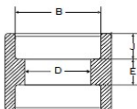
MANICOTTI Couplings
