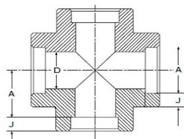
CROCI Crosses
