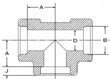
TEE UGUALI Equal tees
