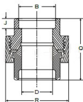
BOCCHETTONE Unions
